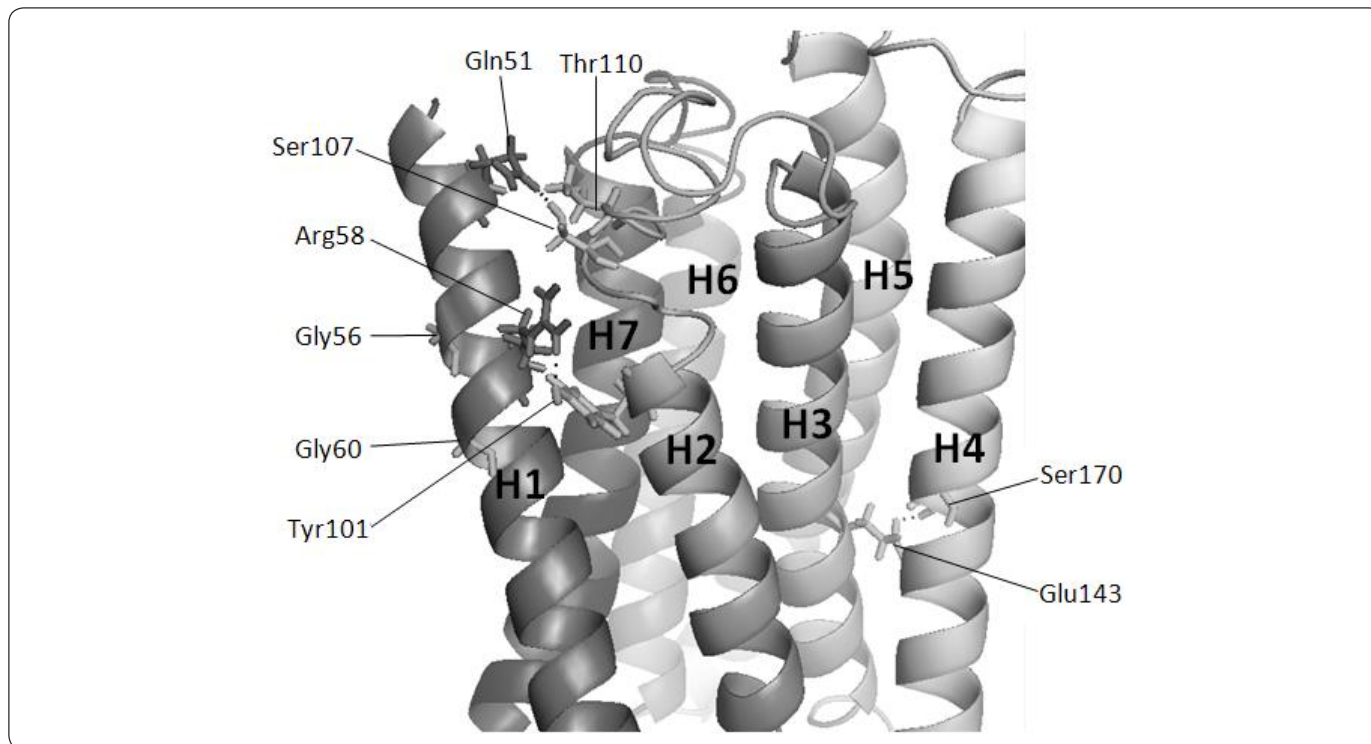
Figure 3. Residues involved in helix-helix interactions in Ste2p model. The transmembrane helices of Ste2p are presented as ribbons and are enumerated from H1 to H7. For convenience, transmembrane helices are displayed in a clockwise orientation. Hydrogen bonds are formed between Arg58-Tyr101, Ser170-Glu143, and Ser107-Gln51-Thr110, and are displayed with dots. Gly56 and Gly60 are oriented outwards the protein. The image was generated with PyMol.
