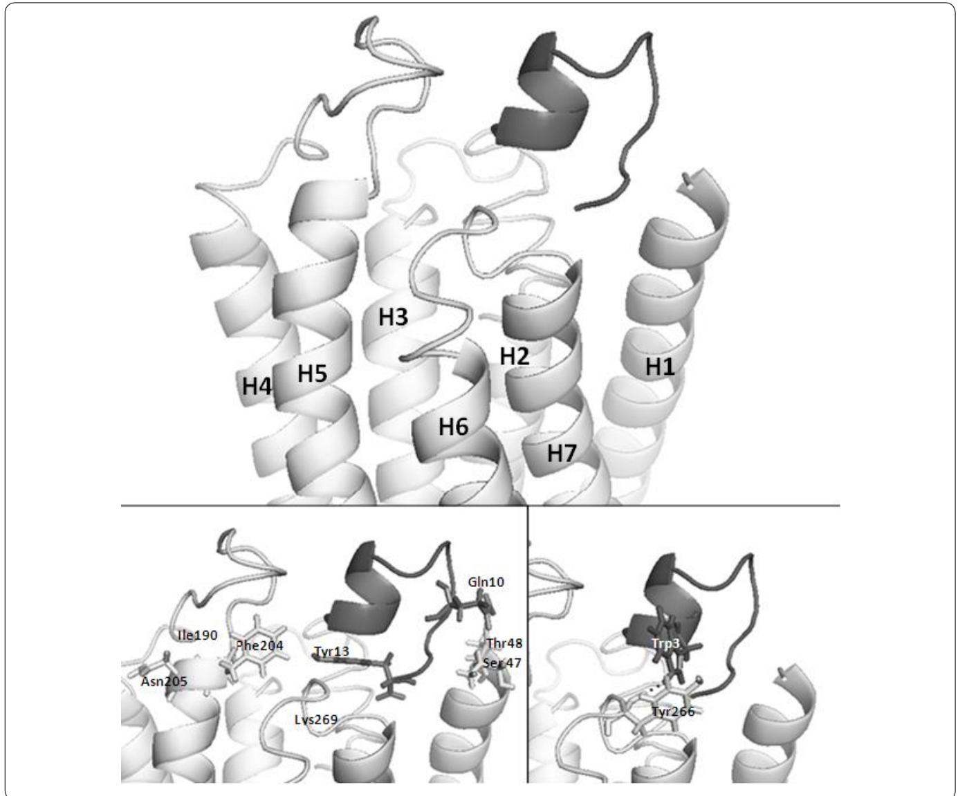
Figure 4. Atomic three-dimensional model of the interaction between Ste2p and the alpha pheromone. Ste2p is shown in a light grey ribbon representation. The alpha pheromone is shown as a dark grey object. The upper part of the figure illustrates the binding pocket formed by extracellular loops and extracellular ends of H1, H5, and H6. In the lower part of the figure, selected residues of Ste2p and pheromone are shown in a ball-and-stick representation. First, the C-terminal region of the pheromone (Gln10) binds to the receptor residues Ser47 and Thr48 (H1) 17 . Then, the central region of the pheromone (Pro8-Gly9) forms a \beta -turn 46 . At this point, Phe204 (H5) is near to Tyr13 in the pheromone 18 , and Lys269 (H6) is near to both the N and C-termini of the pheromone. Asn205 is facing toward the outside of Ste2p and away from the binding pocket (left). In our model, Tyr266 (H6) is oriented towards the surrounding lipids and is inaccessible to solvent. This orientation is consistent with experimental data from 18 . Finally, Tyr266 interacts with Trp3 in the pheromone, mediating the transition to an active state of Ste2 18,47 (right). The image was generated with PyMol.
